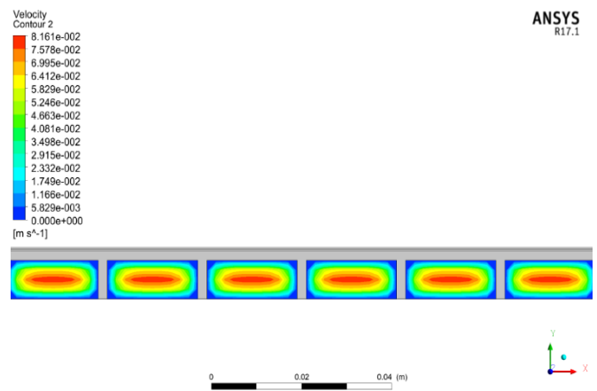
Fig.8. Velocity spectra of fluid flow inside the ducts (case \Phi = 0.06 at Re = 800 ).
